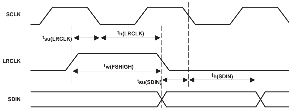
Figure 5-9. DSP Serial Port Timing
